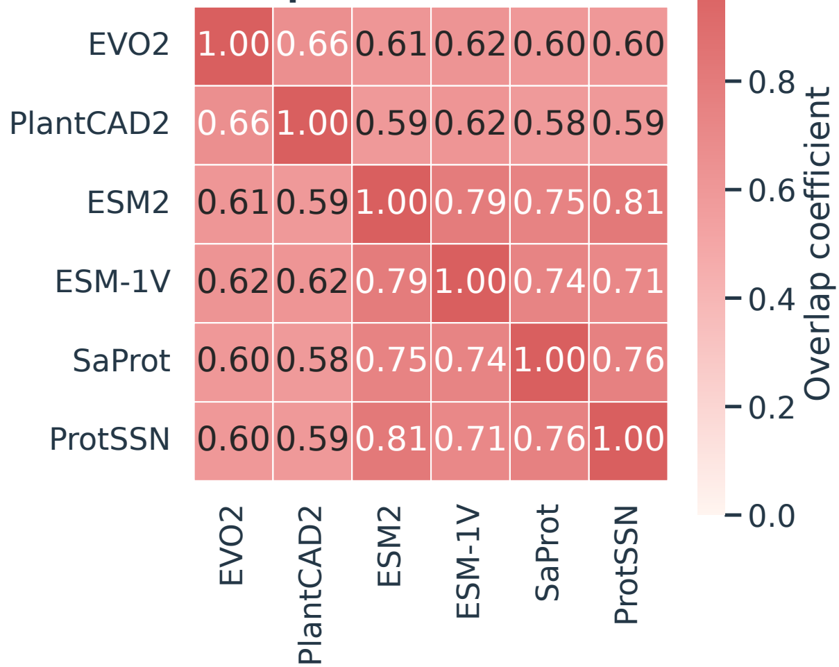
Figure 2D-right. Shared high-risk capture (percentile \geq 75 )
